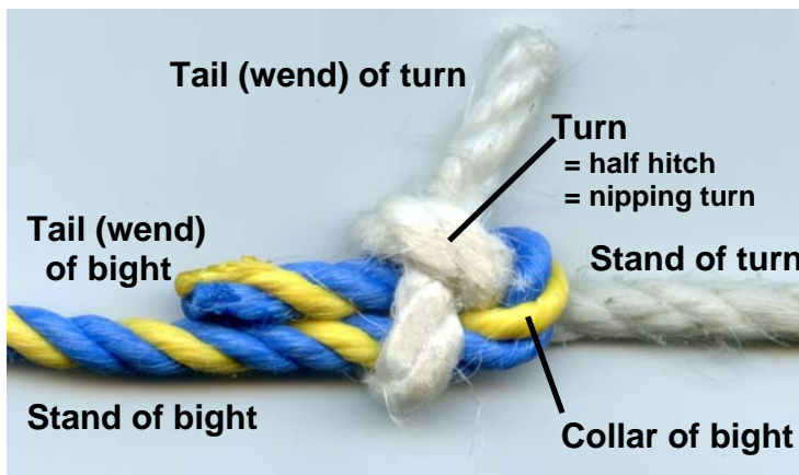
Fig. 1. Single sheet bend with direct tails and S-chirality turn in Z-laid rope.
